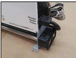
Heater Power Connection
